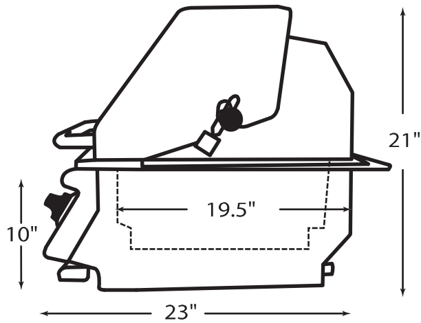
5-Burner Brahma Cut Out Dim. = 38" x 19.5" x 10"
