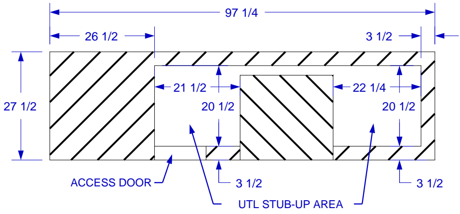
STUB-UP DIAGRAM (SEE NOTE #2)
